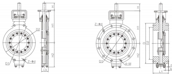
Wafer type Double flanged type
