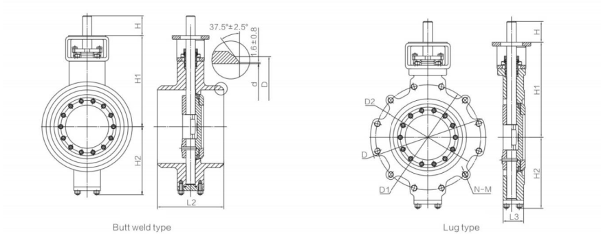
主要连接尺寸 (150LB) Main connecting dimensions
